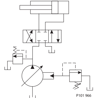
Closed center circuit with remote PC
